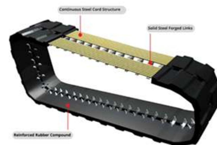
Heavy Duty Construction Rubber Track
